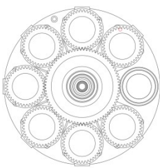
rotating gobo ( Fig.6.2-1 )
